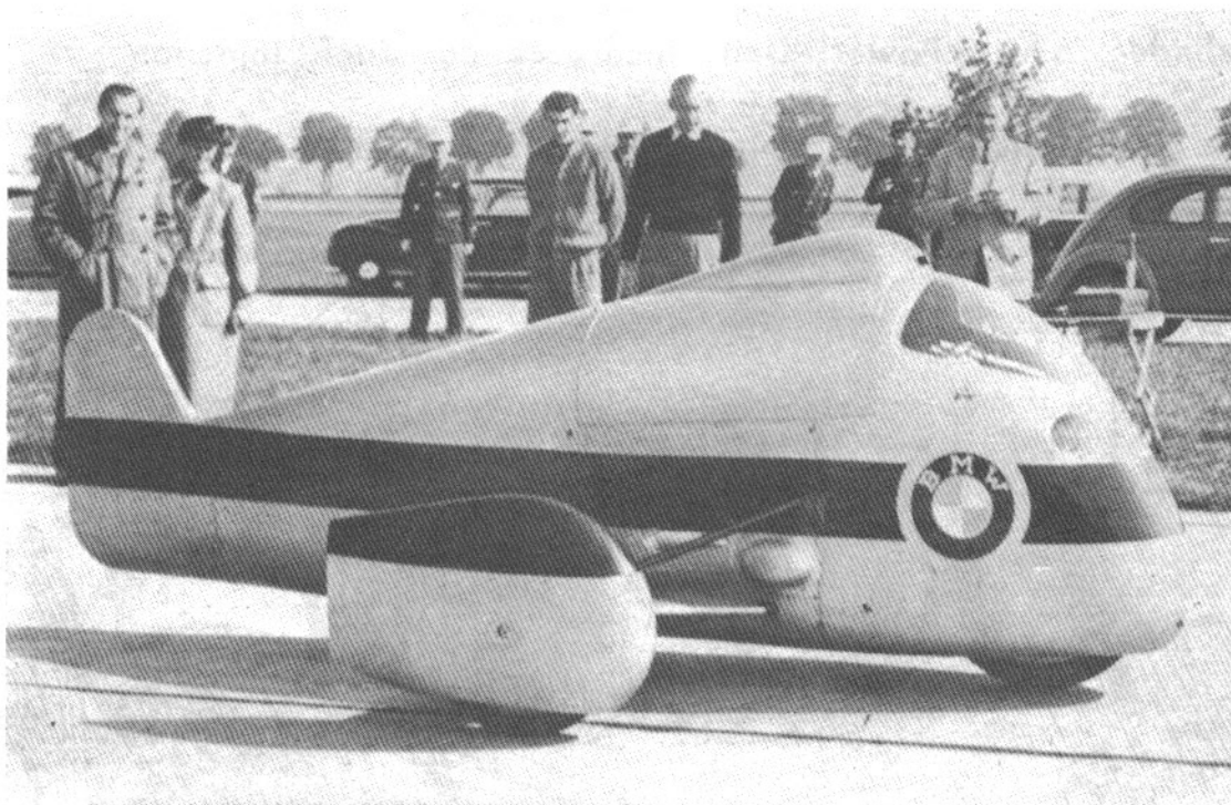
The 500cc B M W, the World's Fastest Sidecar Machine
